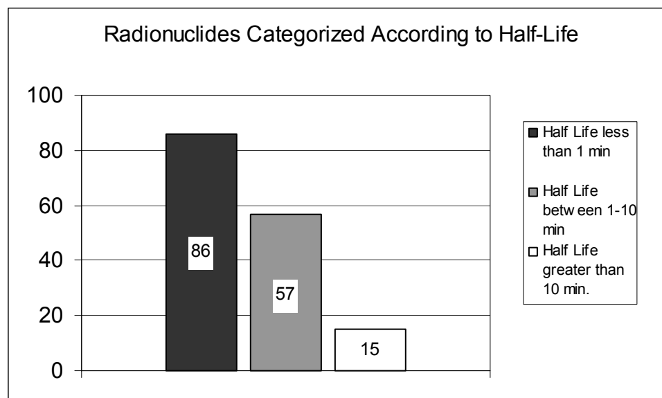
Figure 3.1. Radionuclides identified as lacking a published dose coefficient according to a query of existing radiation safety dose coefficient databases. Seventy two radionuclides with a half-life of greater than or equal to one minute were selected for a dose coefficient evaluation as part of this study.
