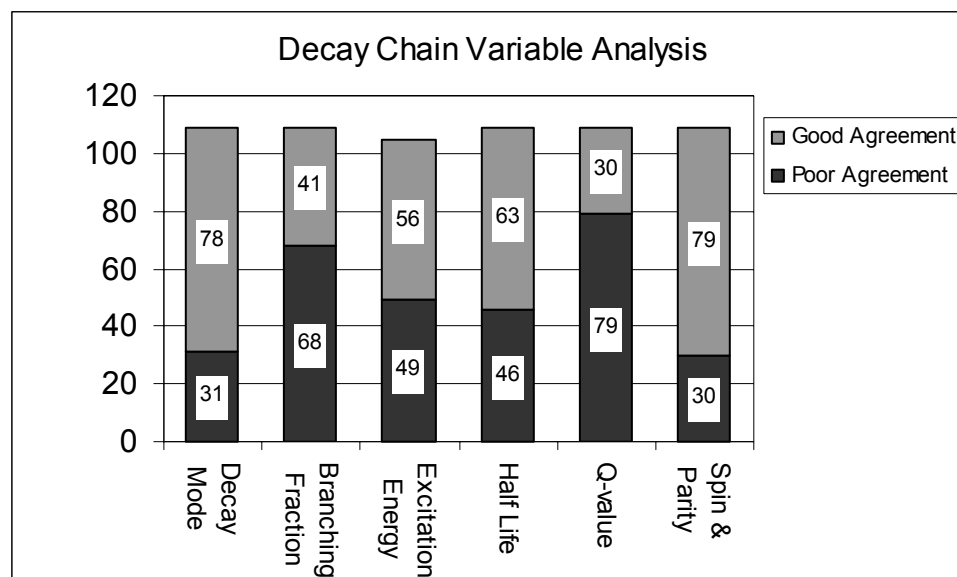
Figure 3.2. Tabulated radionuclidic results for each of the variables evaluated in this work after being cross-referenced and scored.
