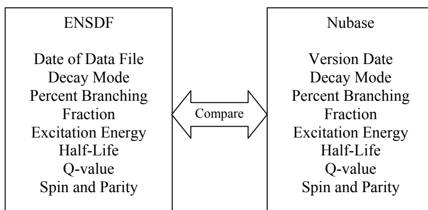
Figure 2.2. Nuclear structure and decay parameters cross referenced between ENSDF and Nubase. ENSDF data files showing good agreement between the databases will be utilized in a dose coefficient calculation.
