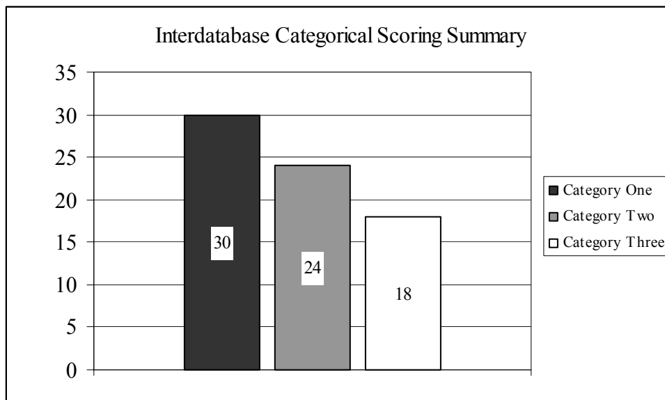
Figure 3.2.2. Categorical scoring summary for the 72 radionuclides identified as lacking a published dose coefficient.
