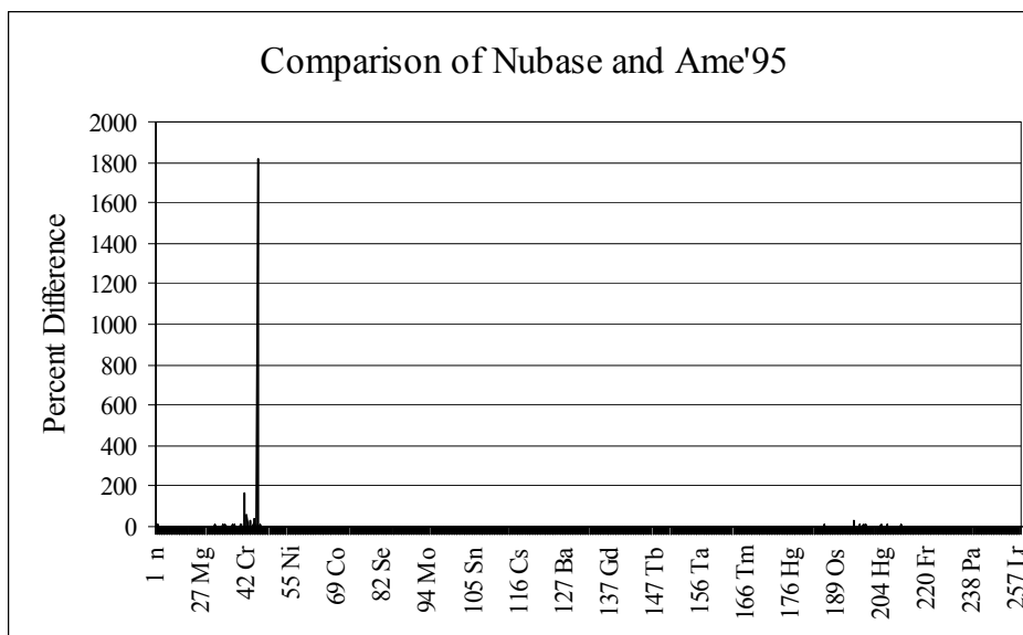
Figure 3.2.1. Comparison of Nubase to Ame'95 showing recent updates to Nubase related to mass excess data.
