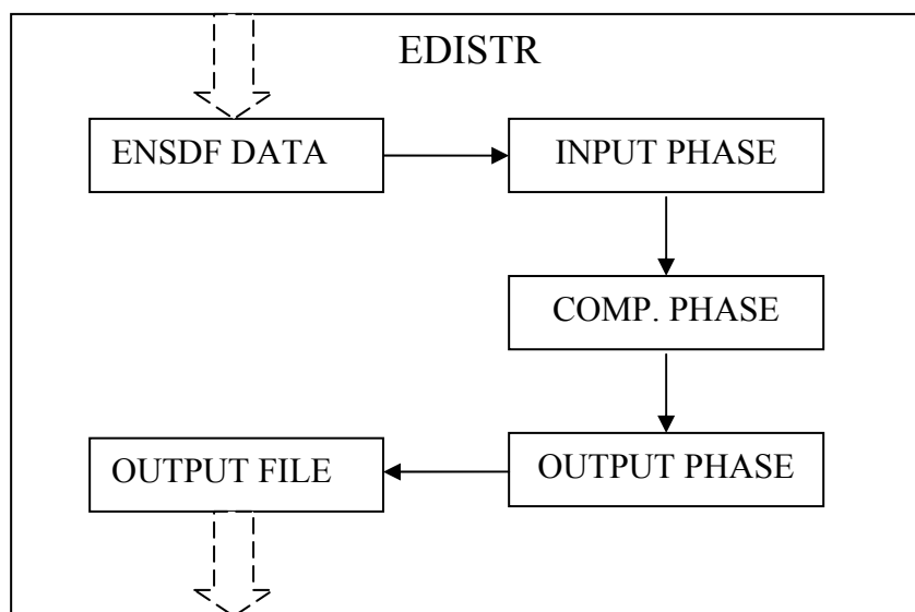
Figure 2.3.1. The three functional phases of the EDISTR code as described by the ORNL/TM-6689 (Dillman 1980).
