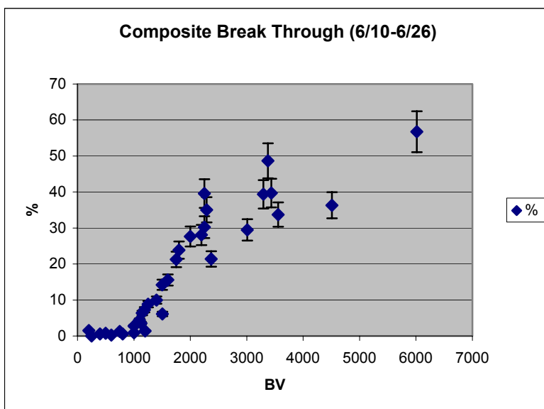
Figure 1.3.2. Percent of iodine in sorbed by Peat columns. The vapor phase was concentration of iodine was 1.2 \cdot 10^{-5} mol/L and was about 50% saturated with nitric acid fumes.
