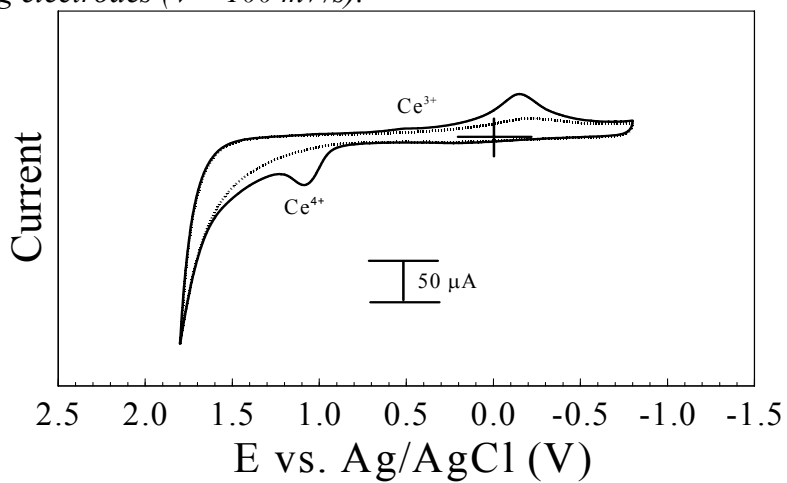
Fig. 3. Comparison of the Ce(III)/Ce(IV) redox couple in 0.1 M \text{HNO}_3 at GC (top), Au, and Pt working electrodes ( \nu = 100 \text{ mV/s} ).
