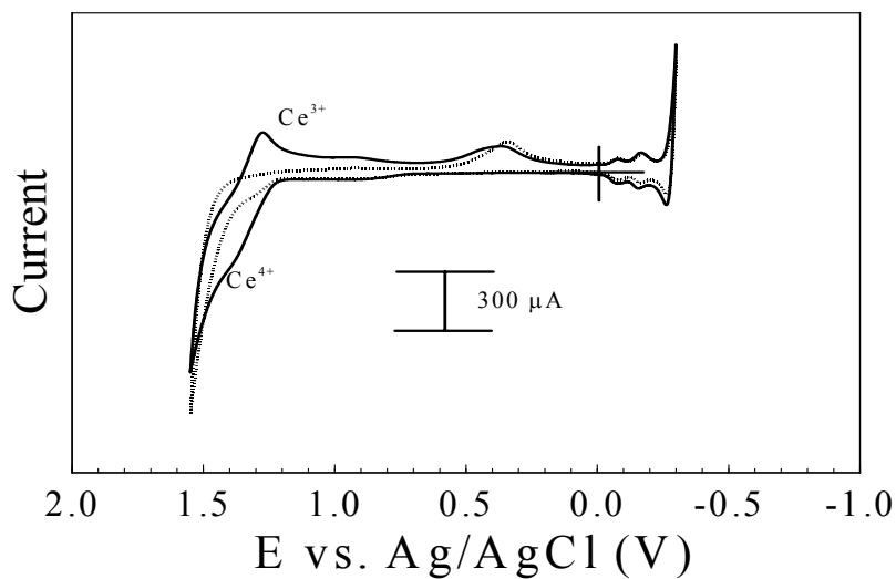
Fig. 3. Comparison of the Ce(III)/Ce(IV) redox couple in 0.1 M \text{HNO}_3 at GC (top), Au, and Pt working electrodes ( \nu = 100 \text{ mV/s} ).
