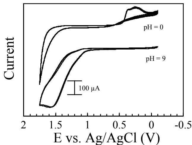
Figure 2. Electrochemistry of Ce(III) at pH = 0 and pH = 9. Scan rate = 100 mV/s.
