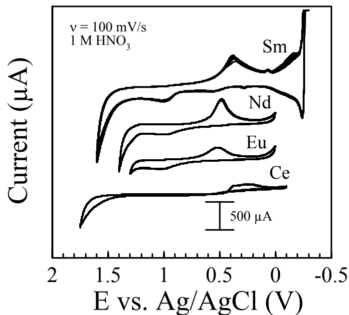
Figure 1. Electrochemical response of a Pt electrode in solution containing 1 \times 10^{-3} M Ce, Eu, Nd, and Sm in 1 M HNO 3 . Scan rate = 100 mV/s.
