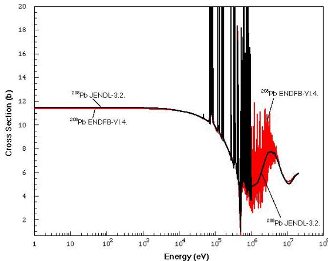
Figure 3 Differences in ENDF/B-6.4 and JENDL-3.2 Elastic Scattering Cross Sections for ^{208}\text{Pb} ( http://fachp1.ciemat.es/texto.html )
