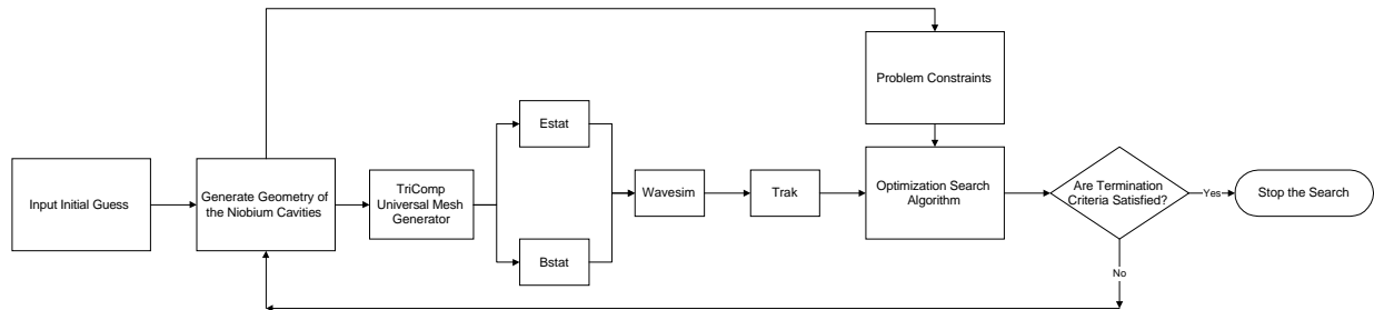
Figure 4. Flowchart for Optimal Design of Niobium Cavities
