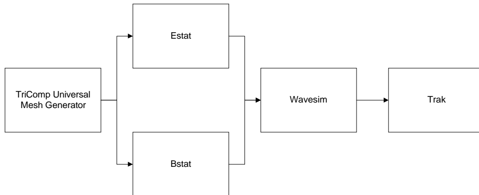
Figure 3. Modeling of Multipacting
