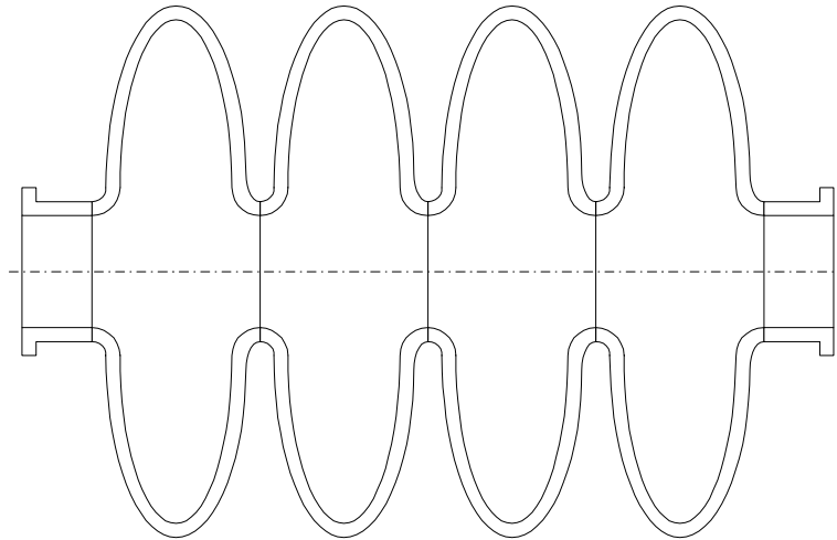
Figure 1. Schematic Diagram of Niobium Cavities
