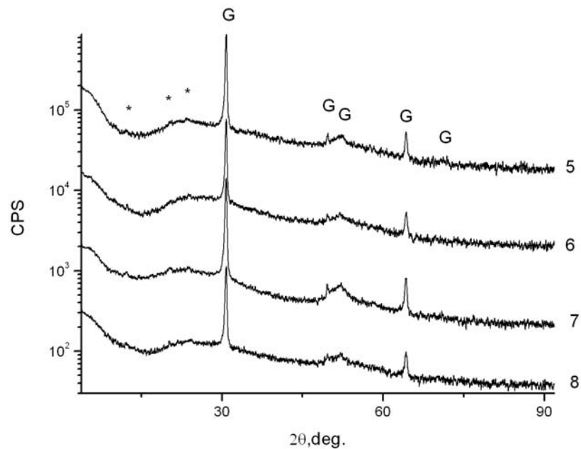
Figure 7. XRD patterns of iodine doped FCC: (5)- initial and (6-8) after interaction with Si-organics under different conditions. Peaks of graphite are marked as “G” and C_{60} as *.
