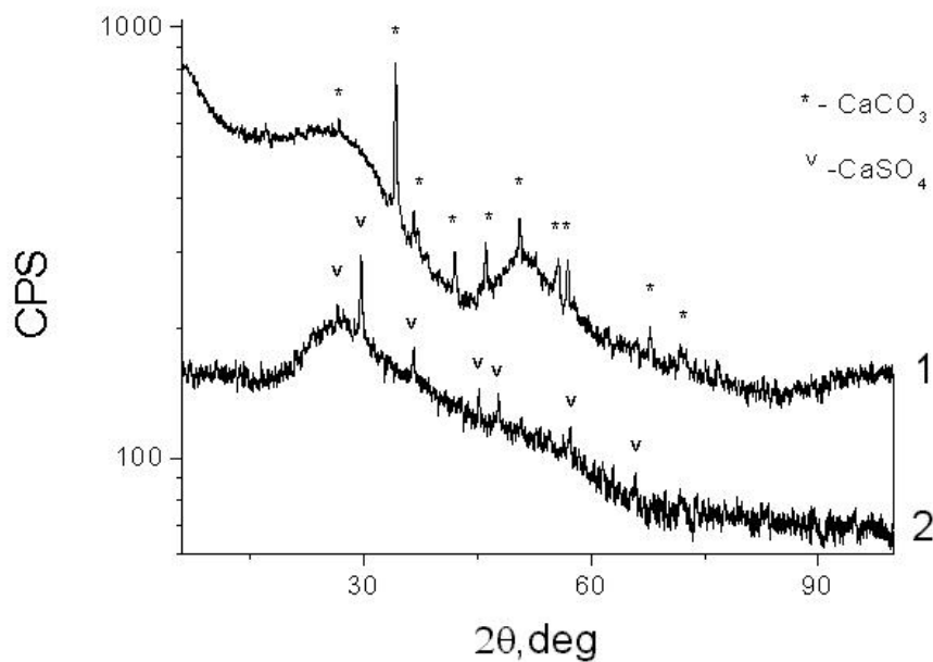
Figure 3. XRD patterns of activated carbon SKT-3S: 1) initial undoped; 2) iodine-doped (571 mg/g). There are no crystalline carbon phases in both samples. Type of activated carbon SKT-3S contains admixtures of calcite (CaCO 3 ) and elemental sulfur that causes formation of anhydride (CaSO 4 ) during process of iodine doping at 300°C.
