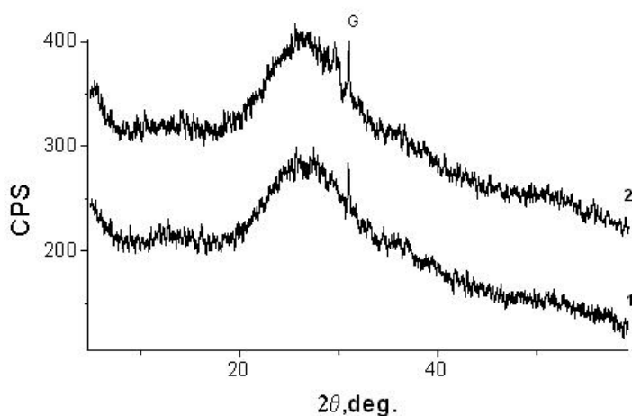
Figure 5. XRD patterns of iodine doped (432 mg/g) activated carbon after gamma-irradiation in nitrogen atmosphere at: 1) 3.3x10 7 Rad and 2) 2.1x10 7 Rad. Reflection of graphite phase is marked as ( G ).
