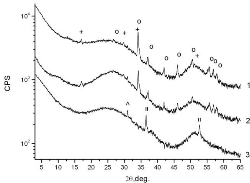
Figure 8. XRD patterns of undoped activated carbon SKT-3S: (1)- initial and (2-3) after interaction with Si-organics under different conditions. Peaks of calcite, \text{CaCO}_3 , are marked as “o”; unknown organic phase as “+”; calcium sulfide, \text{CaS} , - “II” and quartz - “^”.
