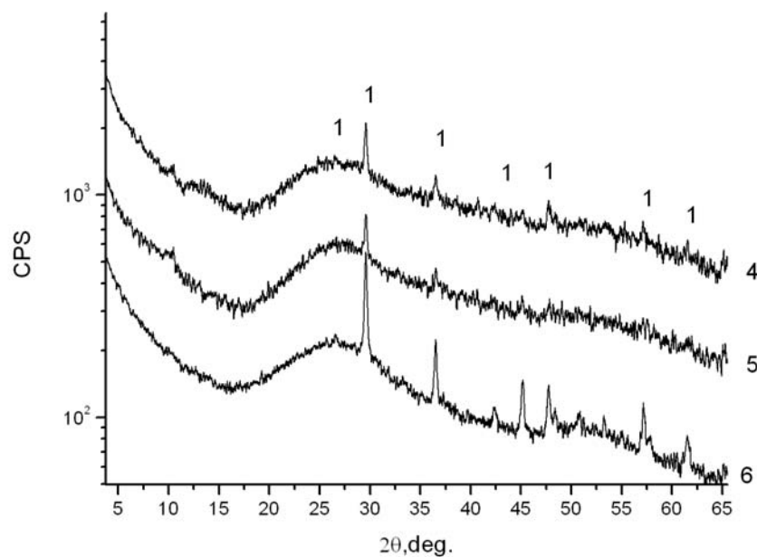
Figure 9. XRD patterns of iodine doped activated carbon SKT-3S: (4)- initial and (5-6) after interaction with Si-organics under different conditions. Peaks of anhydride, \text{CaSO}_4 , are marked as “1”.
