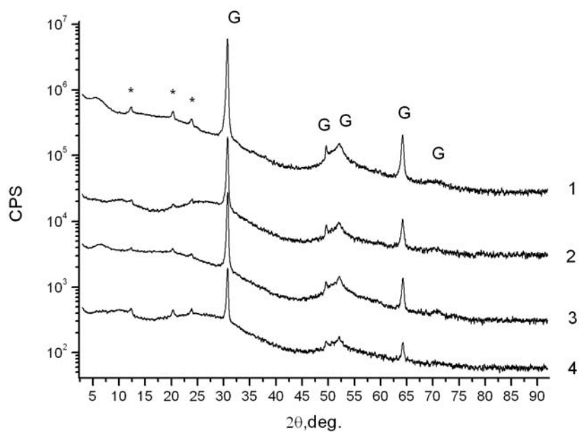
Figure 6. XRD patterns of undoped FCC: (1)- initial and (2-4) after interaction with Si-organics under different conditions. Peaks of graphite are marked as “G” and C_{60} as *.
