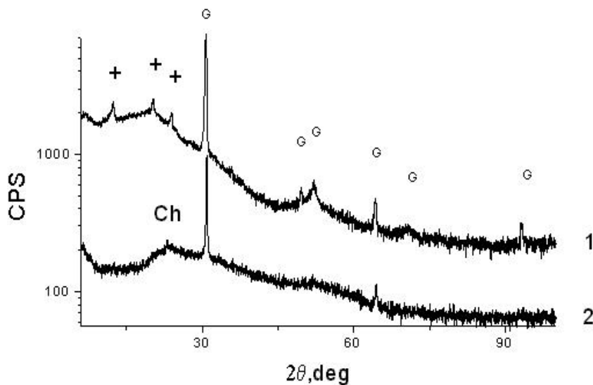
Figure 2. XRD patterns of FCC: 1) initial undoped with fullerene content 6.2 wt.%; 2) iodine-doped (683 mg/g). The following peaks are marked: “G” – graphite; “+” – C 60 ; “Ch” – chaoite.
