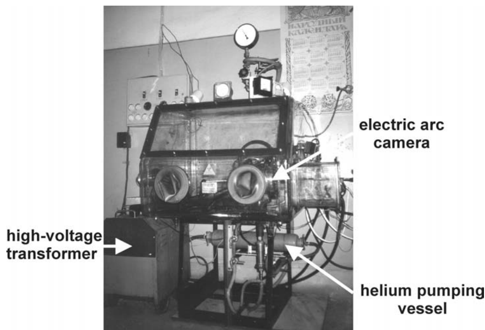
Figure 1. Electric-arc equipment installed into glove box for the synthesis of FCC material.
