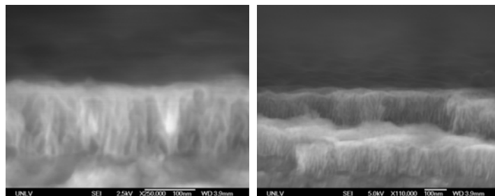
Cross-sectional FESEM images of Ni nanowires electrochemically deposited inside nanoporous alumina for different time lengths.
