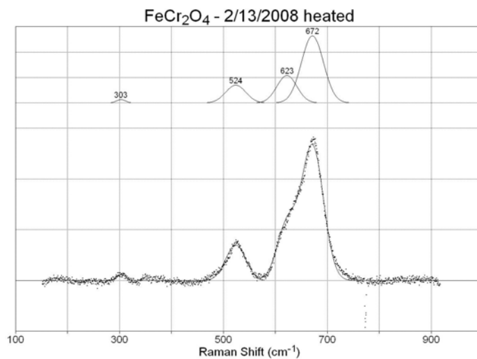
Raman Spectrum of FeCr_2O_4
