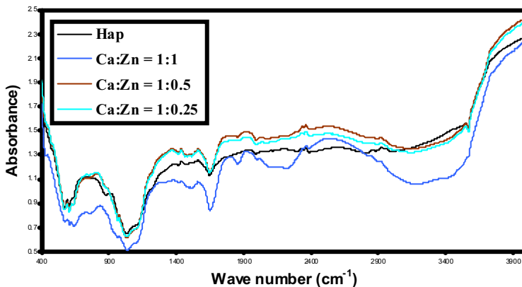
FTIR spectra of samples with different Ca:Zn weight ratios
