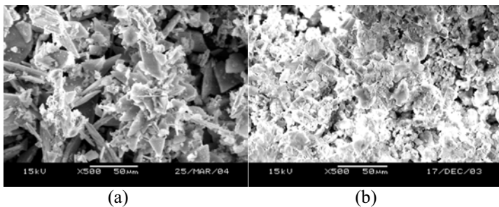
SEM micrographs of synthesized samples with different initial Ca:Zn weight ratios, 1:0.25 (a), 1:1 (b)
