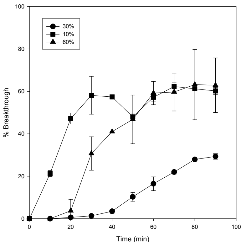
Figure 20: Percent iodine breakthrough for three different Sphagnum Peat/ \text{Ca}(\text{OH})_2 ratios. The trap consisted of \sim 0.5 g of \text{Ca}(\text{OH})_2 : sphagnum mixtures. Three ratios were tested: 10, 30, 60%. The flow rates were 20.0 mL/min and the concentration of iodine was \sim 10^{-5} mol/L. The carrier was 50% saturated with nitric acid vapor. The breakthrough is shown as a function of pore volumes. Pore volumes were estimated by water displacement. The procedure was reported in earlier reports. 40 min corresponds to approximately 1000 pore volumes.
