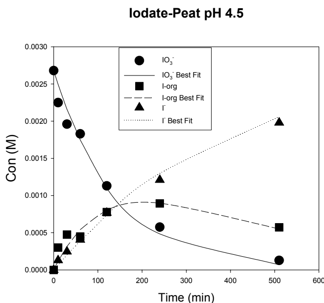
Figure 10: Reaction of \text{IO}_3^- with sphagnum peat at 60°C at pH 4.5. I-org corresponds to the organic bound iodine (substitution) and was calculated by mass balance. Iodate and iodide were measured by ion chromatography.
