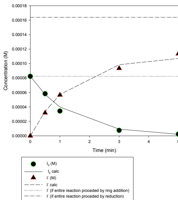
Figure 6: Iodine and Iodine concentrations as a function of time the presence of a suspension of Sphagnum peat (at pH 5.8). The lines represent best-fit results.
