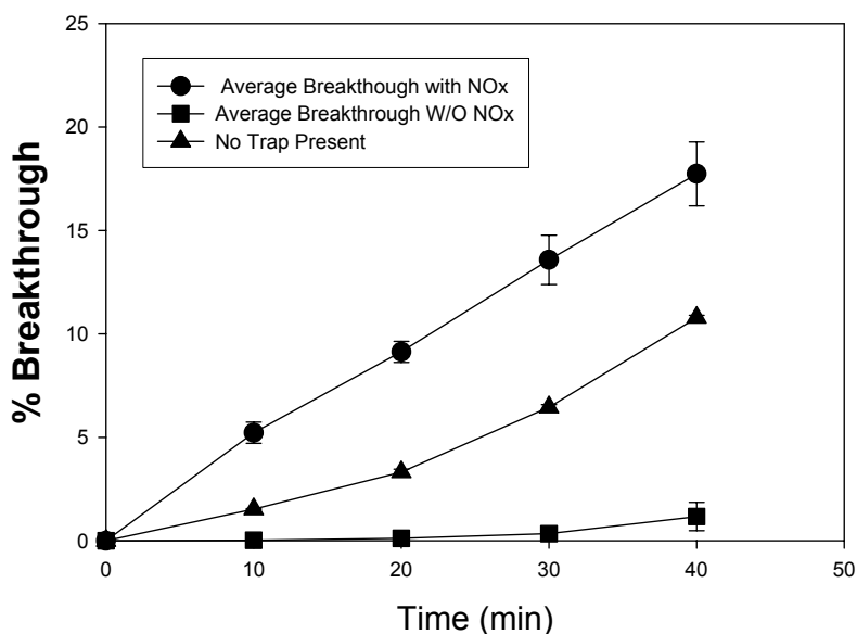
Figure 23: Impact of \text{NO}_2 on iodine breakthrough with sphagnum traps using the fuel rod dissolution apparatus.
