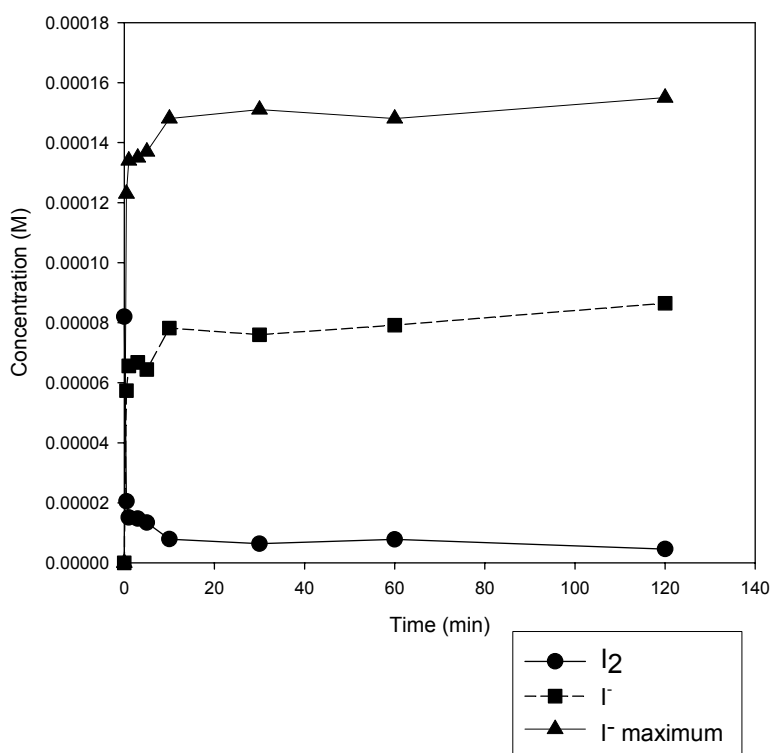
Figure 2: Reaction of iodine with vanillin (40 \mu\text{M} ) at 25 ^\circ\text{C} and pH 2.5.
