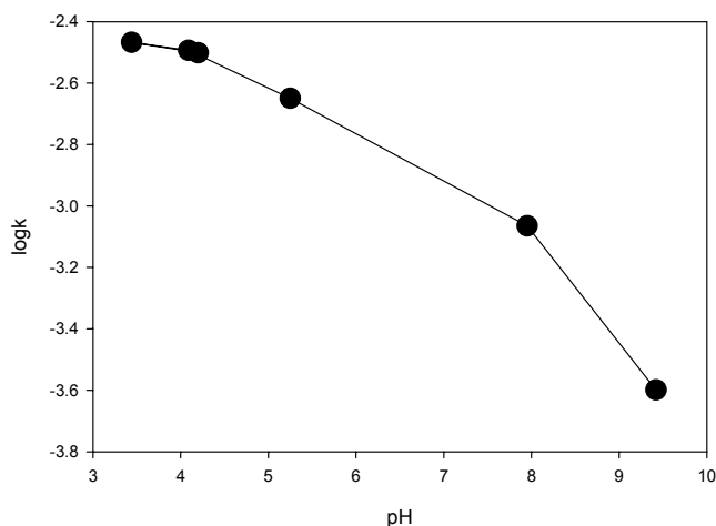
Figure 13: The pseudo first order rate constants for loss of iodate at various pHs at 60°C.
