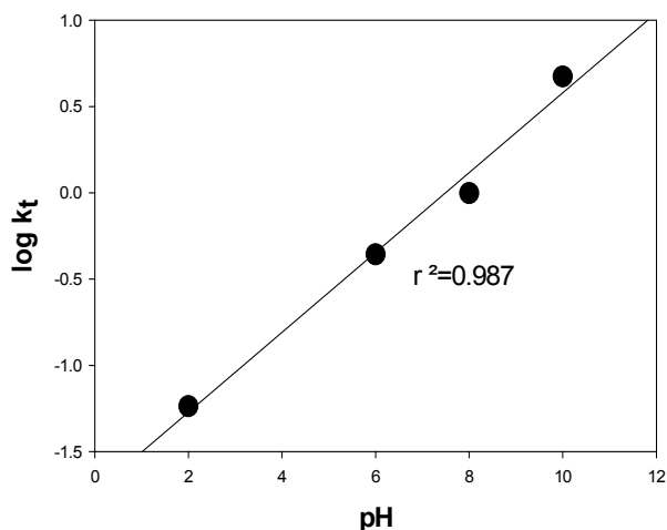
Figure 5: The pseudo first order rate constant for iodine binding as function of pH.
