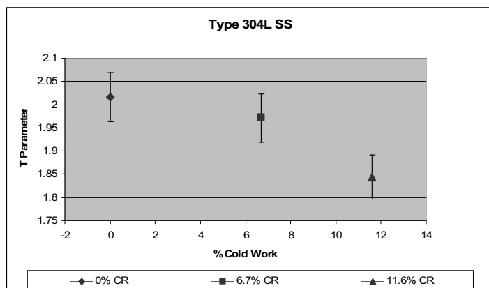
T-Parameter vs Percent Cold Work.
