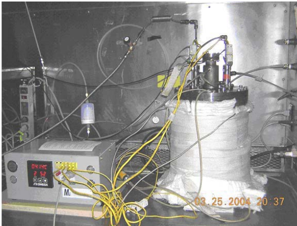
Experimental apparatus developed at UNLV for the testing of the YSZ oxygen sensors.
