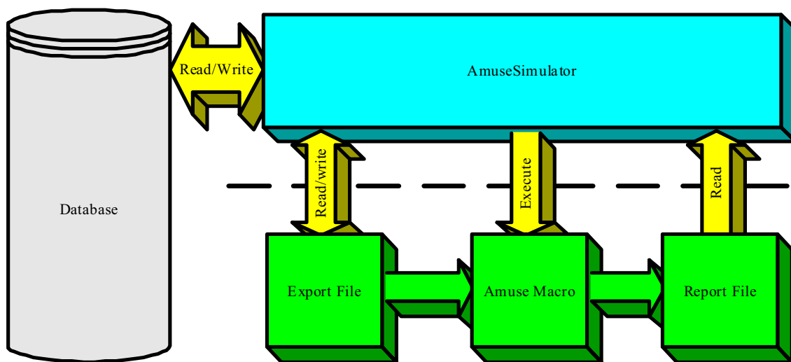
The Architecture design for AMUSE Simulator
