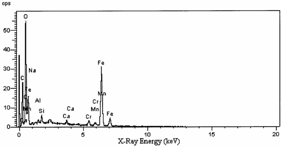
EDAX spectrum of 316 stainless steel, exposed to LBE for 3000 hours at 550 C at IPPE Test Loop.
