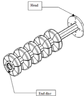
Assembled Optimized UNLV Baffle
