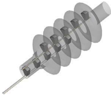
Assembling UNLV Baffle inside cavity
