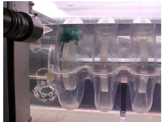
Optimized UNLV Baffle inside cavity
